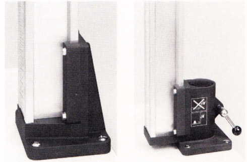
MP-4 Standard (left) has non-rotating column; MP-4 XLR (right) has rotating column.
